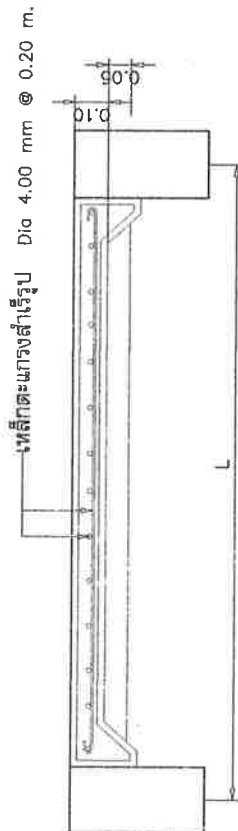
DETAIL GS
